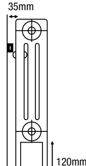
Slip-on Feet
