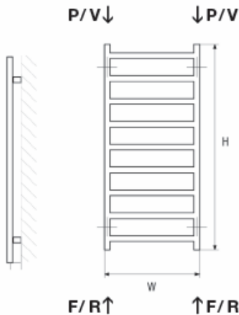
H100 9 Tubes
